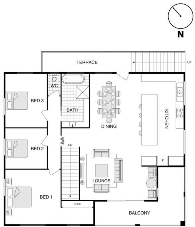
UPPER FLOOR
