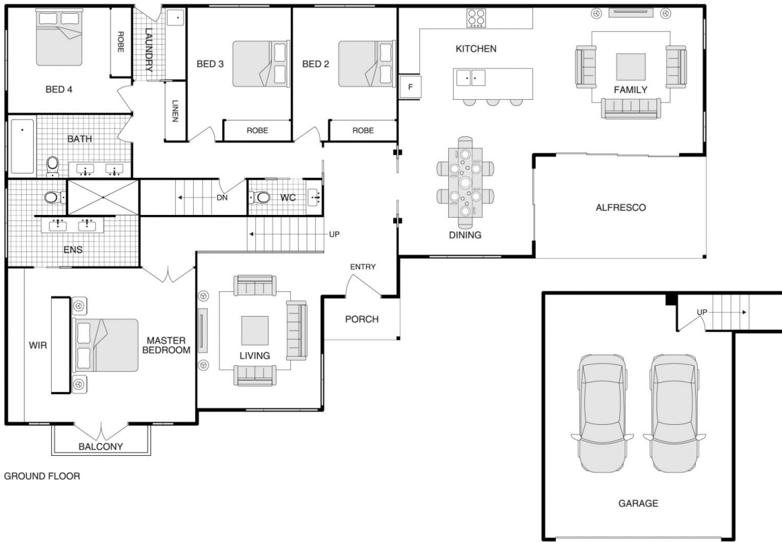
LOWER FLOOR
