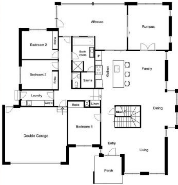
Downstairs
