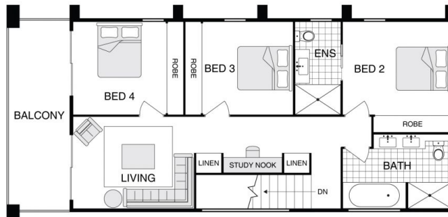
UPPER LEVEL
